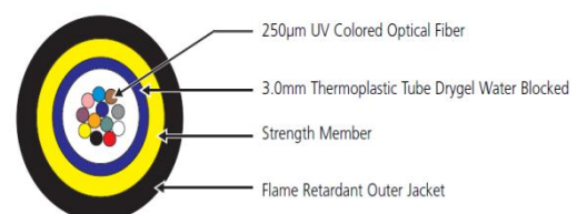
Indoor/Outdoor Dry Loose Tube (up to 12 fibers)
