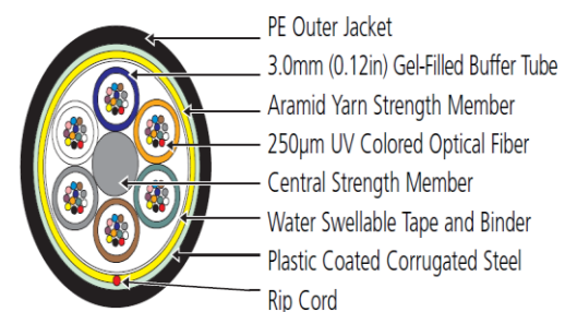
Armored Loose Tube
